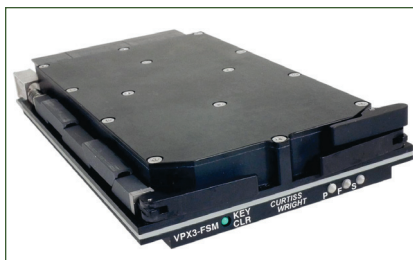
Figure 1 | A 3U VPX SSD
